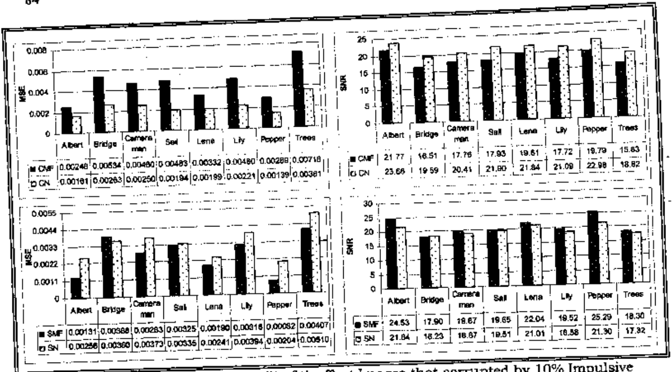
Figure 8: The Average (MSE/SNR) of the Test Images that corrupted by 10% Impulsive Noise and filtered by different Neural Network Schemes together with the Ordinary Median Filter.
